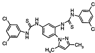
Compound # 39
